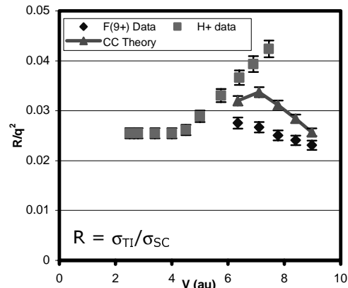
Fig.2. A scaled ratio of transfer ionization to single capture for bare projectiles incident on He. Included are the data of the present work, data of Mergel et al. 3 and a coupled channel calculation for F^{9+} on He.
