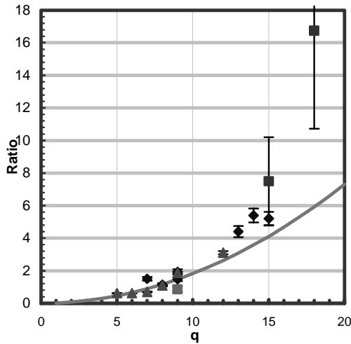
Fig. 1. The ratio of the TI to SC cross sections for dressed and bare projectile ions incident on He is shown. The data included in the paper by Montenegro et al. 2 , are given together with the present results (triangles).
